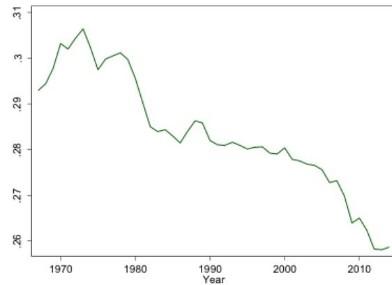
Figure 2. Ratio of log-transformed CO2 emissions to log-transformed GDP per capita for the United States, 1967-2014. Note: original figure based on World Bank data (WB, 2017).
